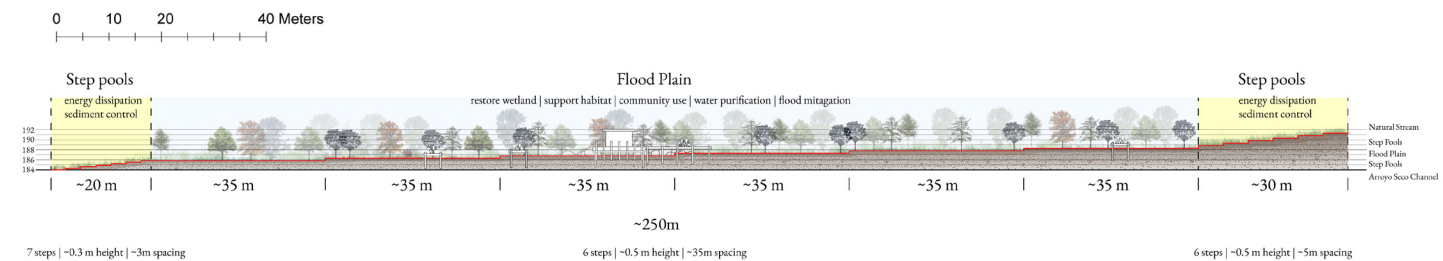
Longitudinal section of a conceptual alternative, showing elevation change across the full corridor.
